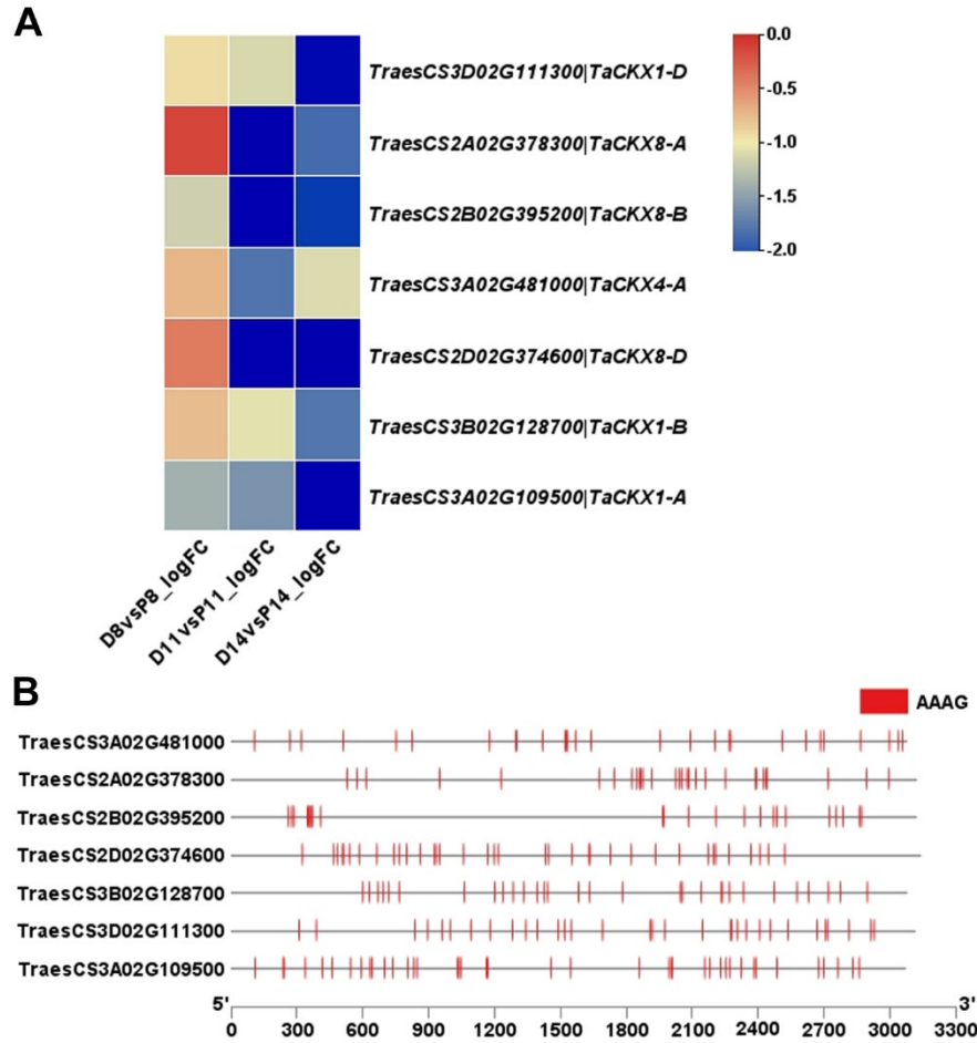
Figure S5. The expression level and motif analysis of the selected CKXs. (A) Expression heatmap of the CKXs in cluster 4 and cluster 5. (B) Motif analysis of the promoters of the selected CKXs. The red vertical lines indicate the possible binding sites of DOF transcription factors.
