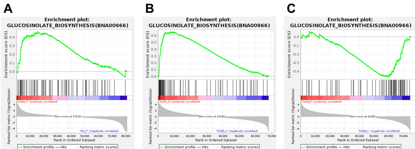
Supplementary Fig. S2 The Gene Set Enrichment Analysis (GSEA) of differentially expressed genes between R2260-Westar (We), among the tissues of leaves (L), flowers (F), silique pericarps (Si) and seeds (Se).
