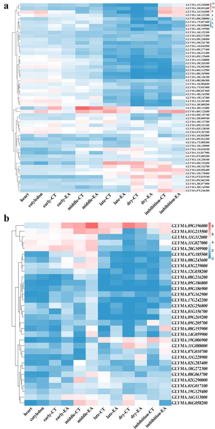
Supplemental Figure S4. Metabolite synthesis during soybean embryo development. (a-b) Heatmap of gene expression patterns from fatty acid (a) and steroid (b) synthesis networks during embryo development.
