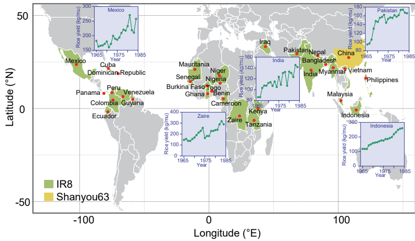
Supplementary Figure 5. The planting region of IR8 and Shanyou63. Green color on the map represents the planting areas of IR8, while orange represents the planting areas of Shanyou63; the broken line represents the yield of rice (yields for some countries are shown on the map).
