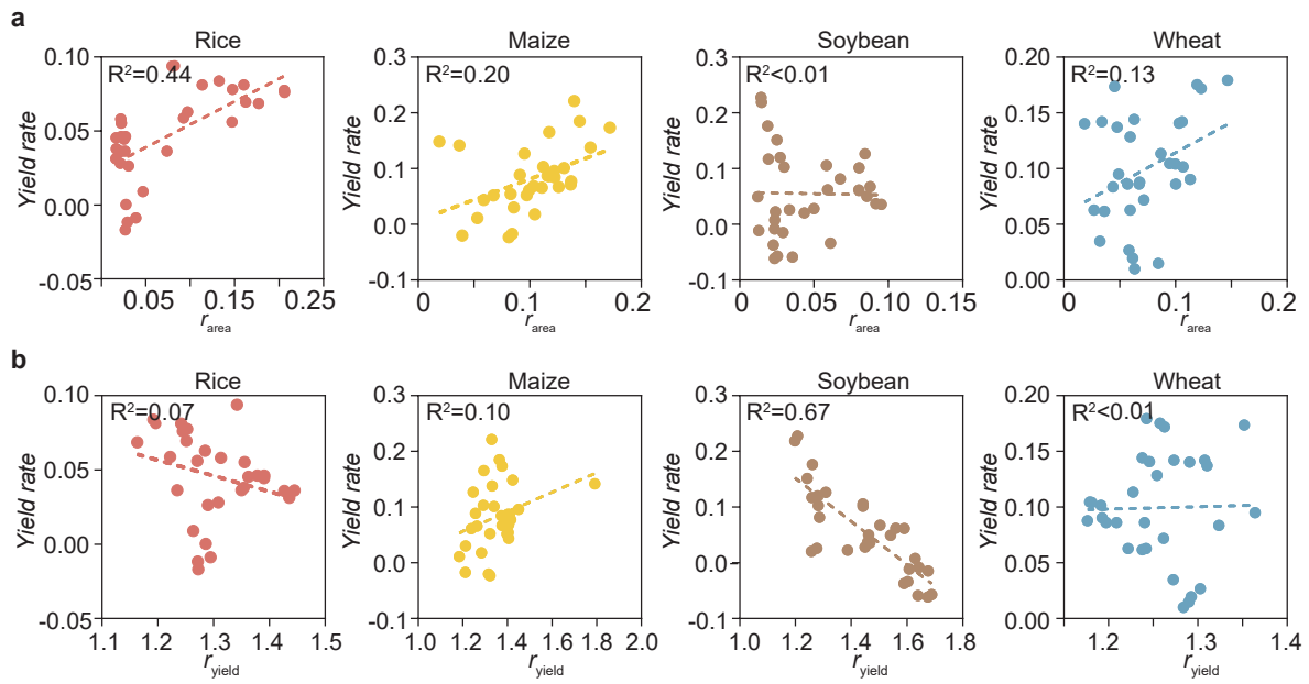
Supplementary Figure 1. r_{\text{area}} and yield rate show a weak positive correlation across global regions. (a) Correlation analysis of r_{\text{area}} with yield rate for rice, maize, soybean, and wheat in global regions. (b) Correlation analysis of r_{\text{yield}} with yield rate for rice, maize, soybean, and wheat in global regions.
