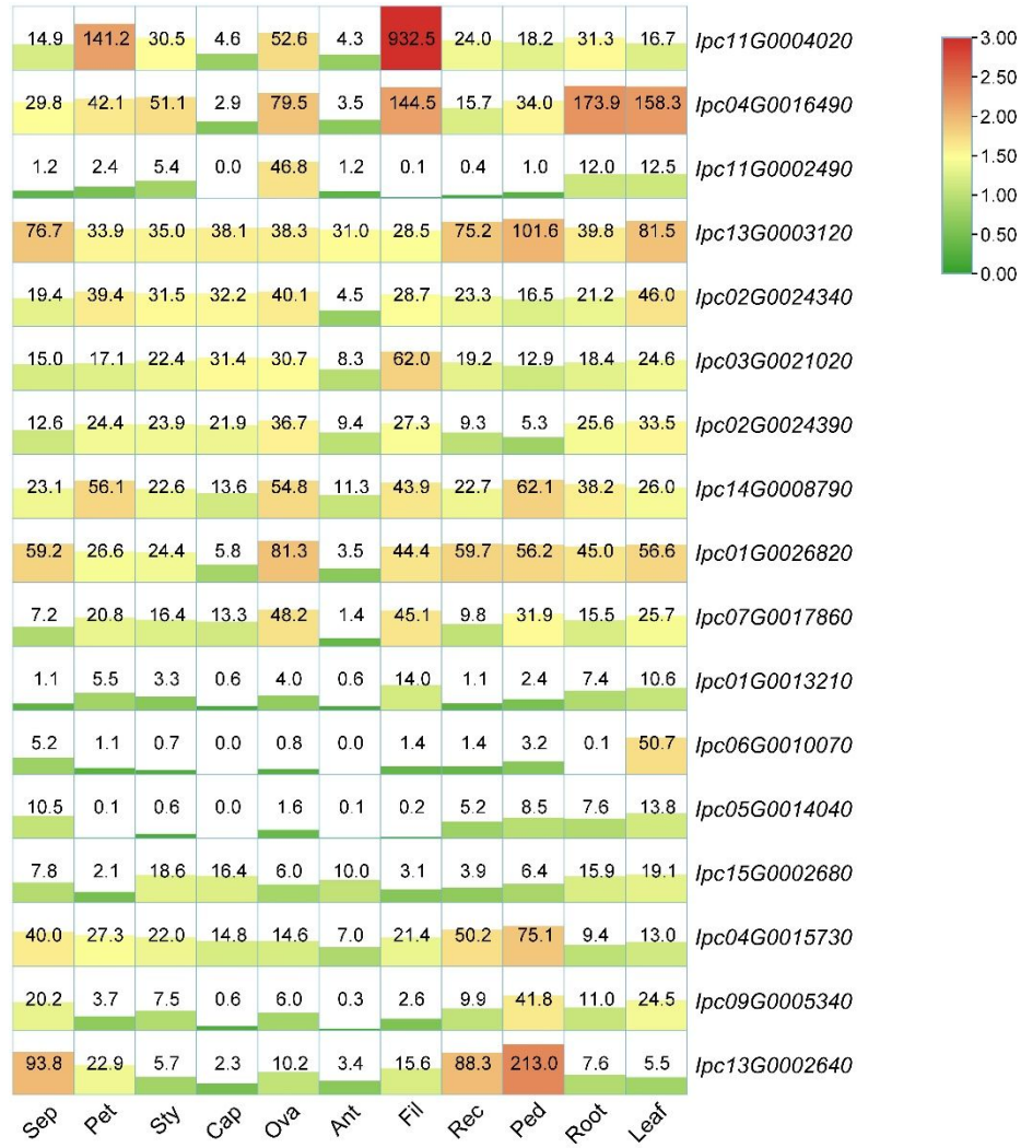
Figure S11. The expressions of quinic acid synthesis genes in different tissue.
