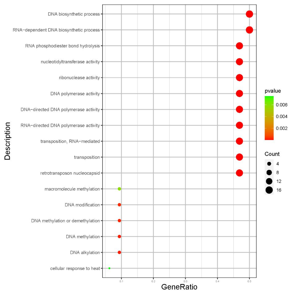
Figure S6. The enriched GO with the TE-associated expanded genes.
