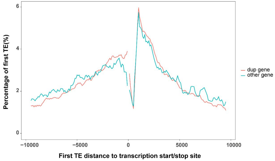
Figure S5. Percentage of nearest TE to transcription start/stop site.
