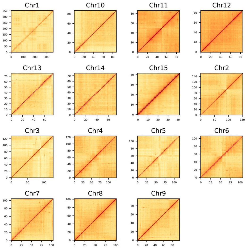
Figure S1. Hi-c integrating map of IPCgenome.
