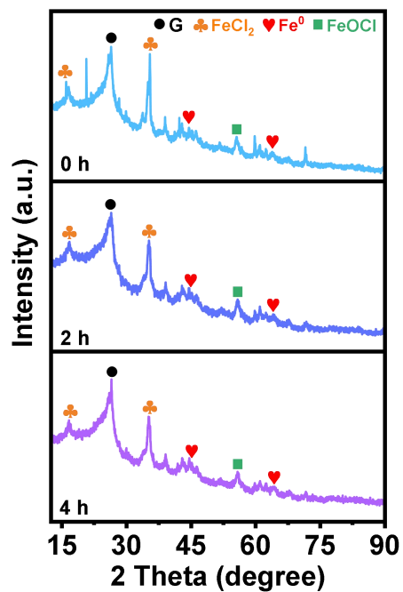
Figure S10. X-ray diffraction spectra of Fe/C-250V composite catalyst at different reaction times (Reaction conditions: SMX = 10 mg/L, Fe/C-250V catalyst = 1.0 g/L, pH = 7, temperature = 298 K).
