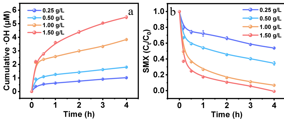
Figure S5. (a) Cumulative \bullet\text{OH} and (b) the removal efficiency of SMX of Fe/C-250V composite catalyst with different dosages.
