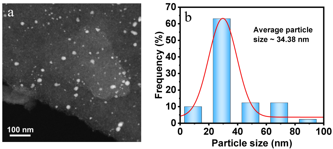
Figure S2. (a) High-angle annular dark-field (HAADF) images and (b) size distribution histogram of Fe particle in Fe/C-250V composite catalyst.
