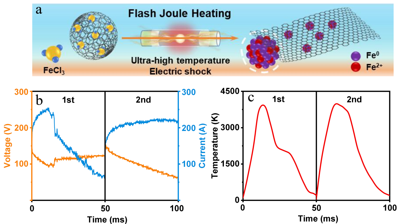
Figure S1. (a) Schematic diagram of the process of preparing Fe/C catalysts by flash Joule heating (FJH) technology. (b) Recording of (b) voltage, current and (c) temperature changes of the synthesized Fe/C-250V composite catalyst during the FJH reaction.
