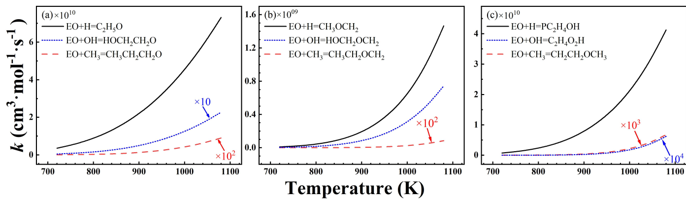
Fig. S1. Rate constants of backside attack reactions by H atom, OH, and CH 3 on EO in the temperature range of 720–1,080 K at 1 atm.
