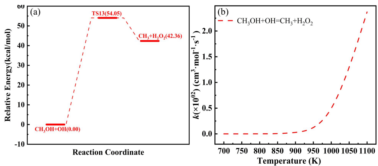
Fig. S3. (a) Potential energy profiles of backside attack reactions by OH atom on \text{CH}_3\text{OH} and (b) the corresponding rate constants in the temperature range of 700–1,100 K at 1 atm.
