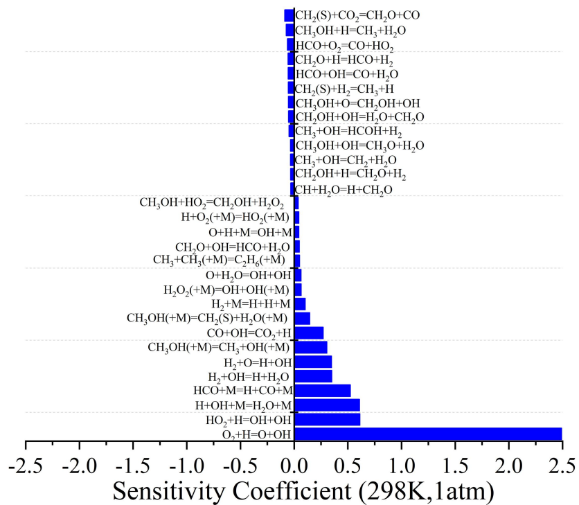
Fig. S7. Sensitivity analysis of methanol for laminar burning velocity at 298 K, \Phi = 1.4 , and 1 atm.
