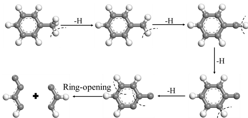
Supplementary Fig. S6. Schematic diagram of toluene molecular cracking pathway.
