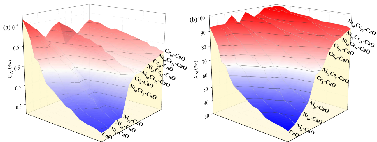
Supplementary Fig. S4. (a) CO 2 absorption capacity and (b) carbonation conversion of Ni and Ce doped CaO materials.
