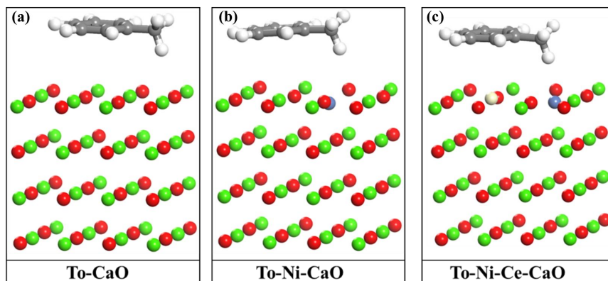
Supplementary Fig. S5. Toluene adsorption configurations on (a) CaO, (b) Ni-CaO, and (c) Ni-Ce-CaO surfaces.
