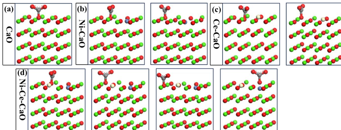
Supplementary Fig. S2. \text{CO}_2 adsorption configurations on (a) \text{CaO} , (b) \text{Ni-CaO} , (c) \text{Ce-CaO} , and (d) \text{Ni-Ce-CaO} surfaces.
