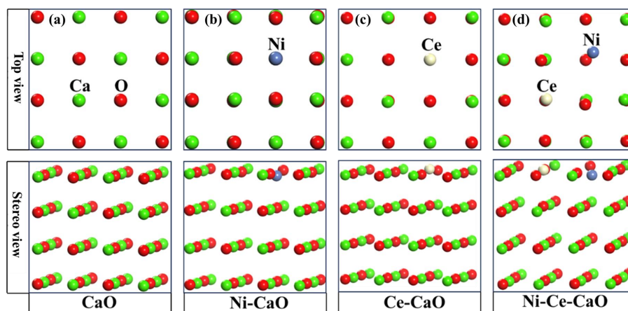
Supplementary Fig. S1. Periodic slab representations of (a) CaO, (b) Ni-CaO, (c) Ce-CaO, and (d) Ni-Ce- CaO surfaces (color scheme: green = Ca, red = O, blue = Ni, gray = Ce).
