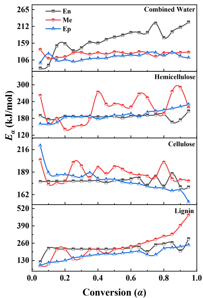
Fig. S7 Relationship between the independent E_a of each component and the conversion rate.
