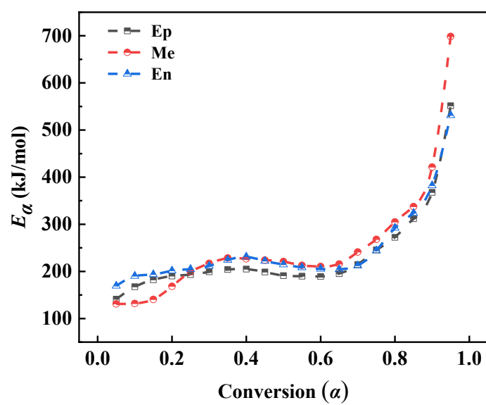
Fig. S6 The curves of activation energy with conversion.
