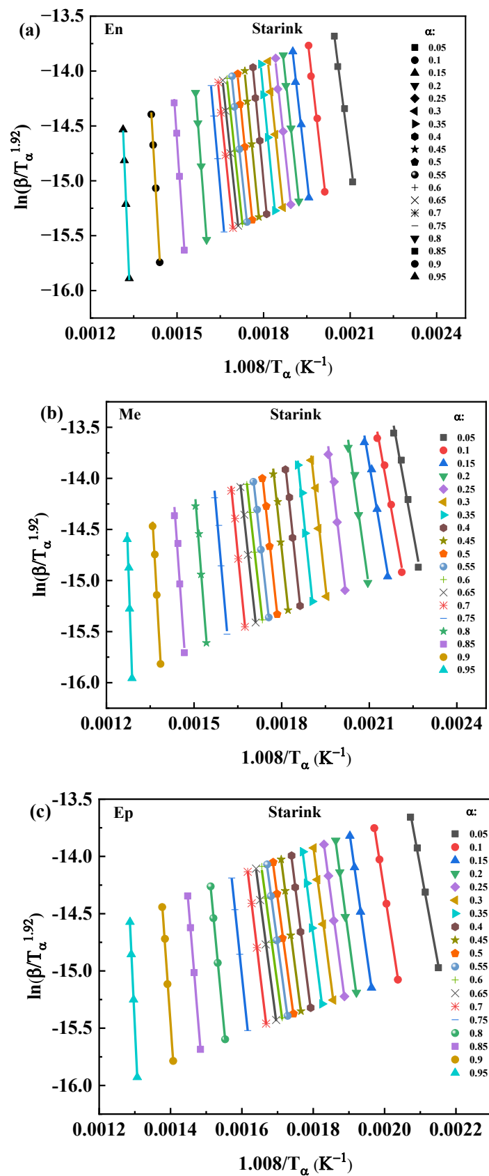
Fig. S5 Linear fitting results of coconut husk wastes by Starink isoconversional methods.
