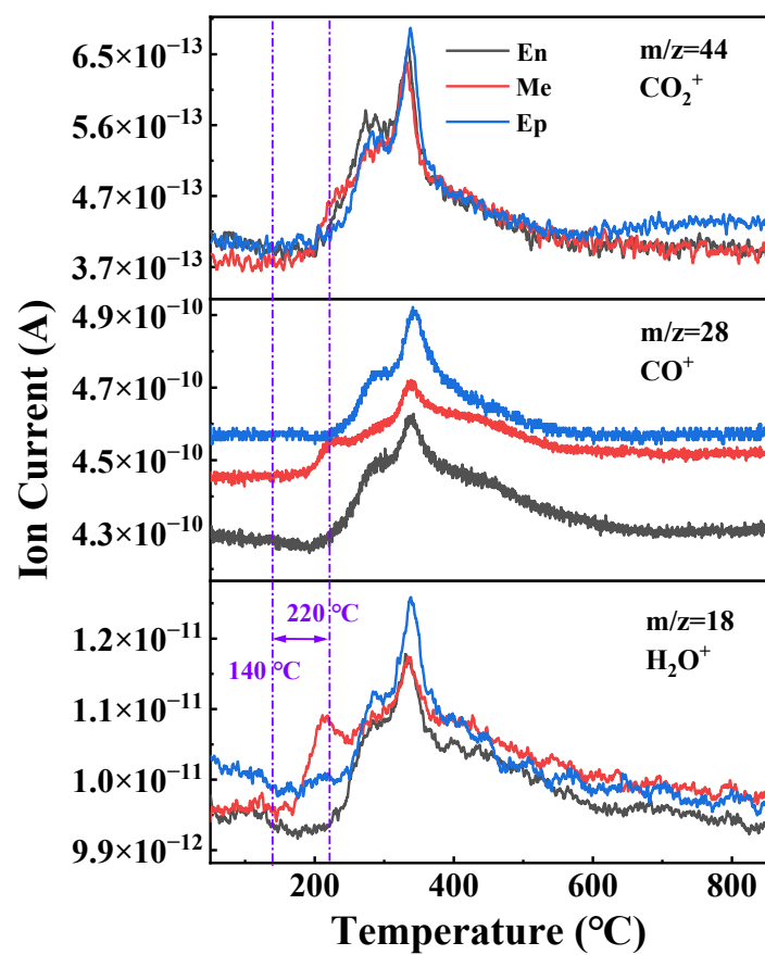
Fig. S3 MS curves of gaseous components from coconut wastes pyrolysis.
