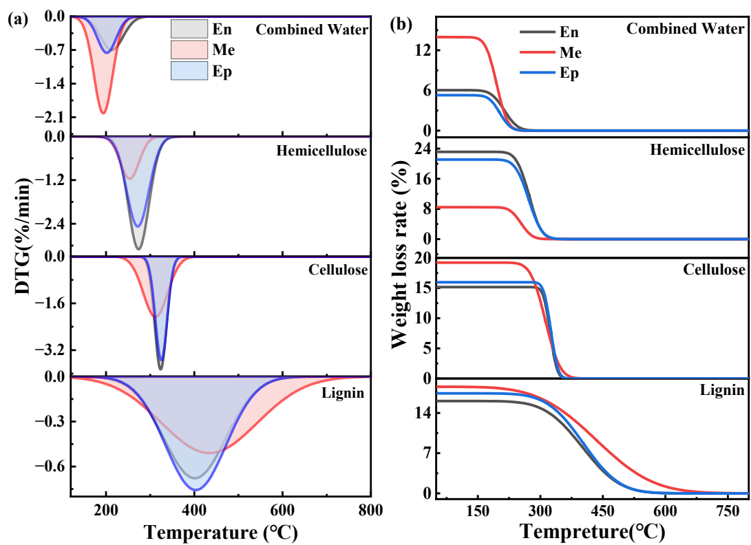
Fig. S2 DTG and weight loss rate curves of each component: (a) DTG; (b) weight loss rate.
