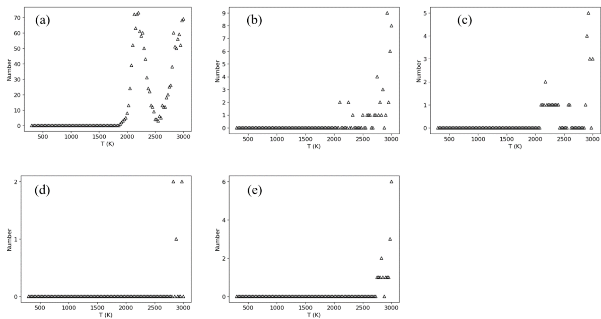
Figure S3. Evolution of C_{11}\sim C_{20} partial products from PP pyrolysis at 1 K/ps. (a): olefins (b): three-membered-ring hydrocarbon (c): five-membered-ring hydrocarbon (d): six-membered-ring hydrocarbon (e): aromatic hydrocarbon
