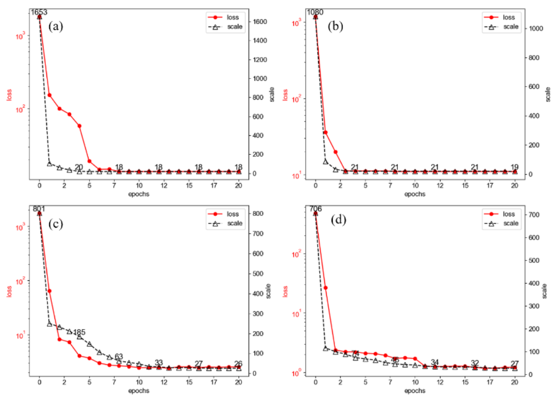
Figure S2. Evolving trends of reaction quantity and loss function during optimization process for PP pyrolysis: (a) 1 K/ps; (b) 2 K/ps; (c) 4 K/ps; (d) 8 K/ps
