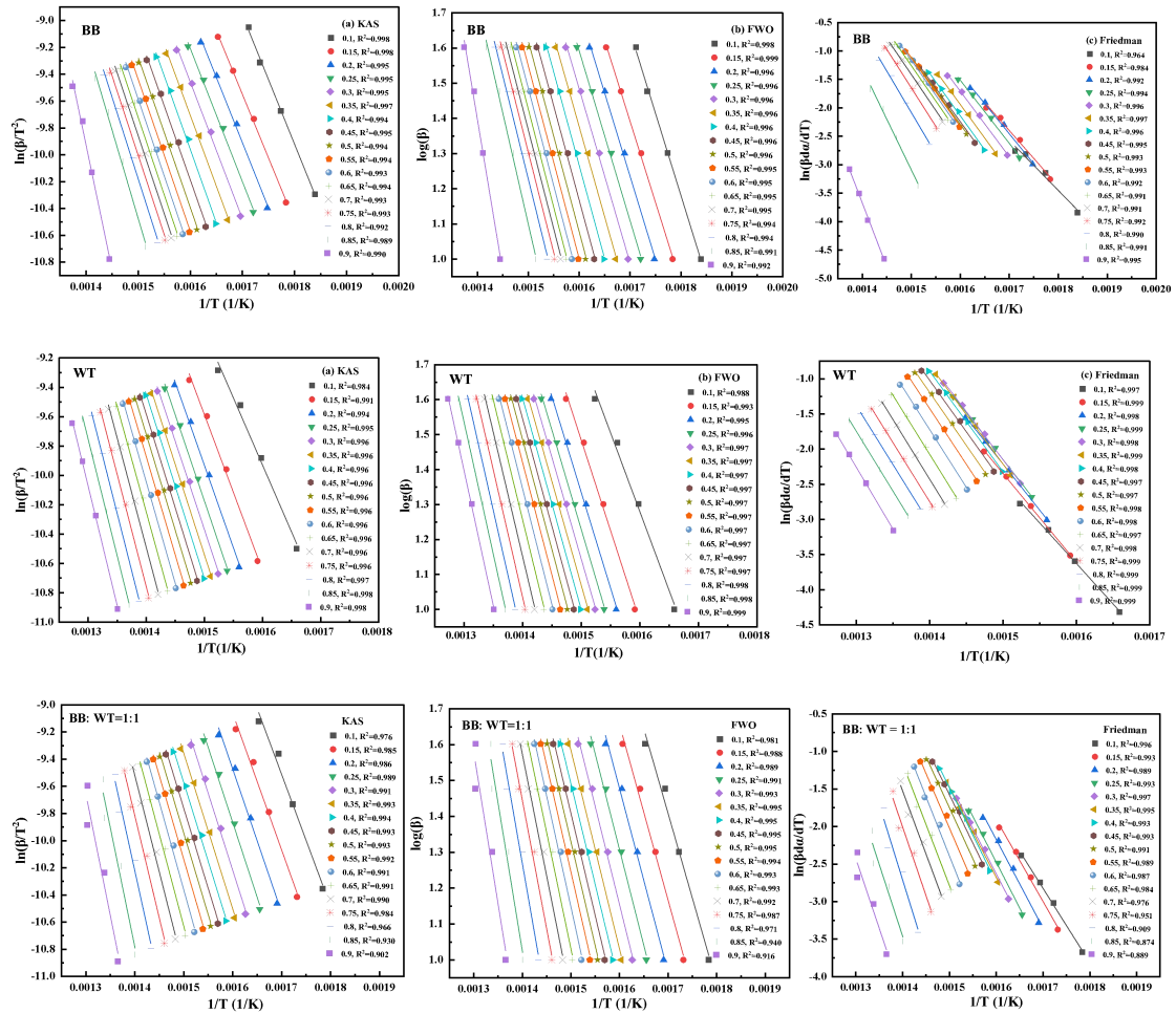
Fig.S3 Linear fitting plots to calculate the E_\alpha of the BB, WT and 1:1 BB-WT blend using KAS, FWO and Friedman models.
