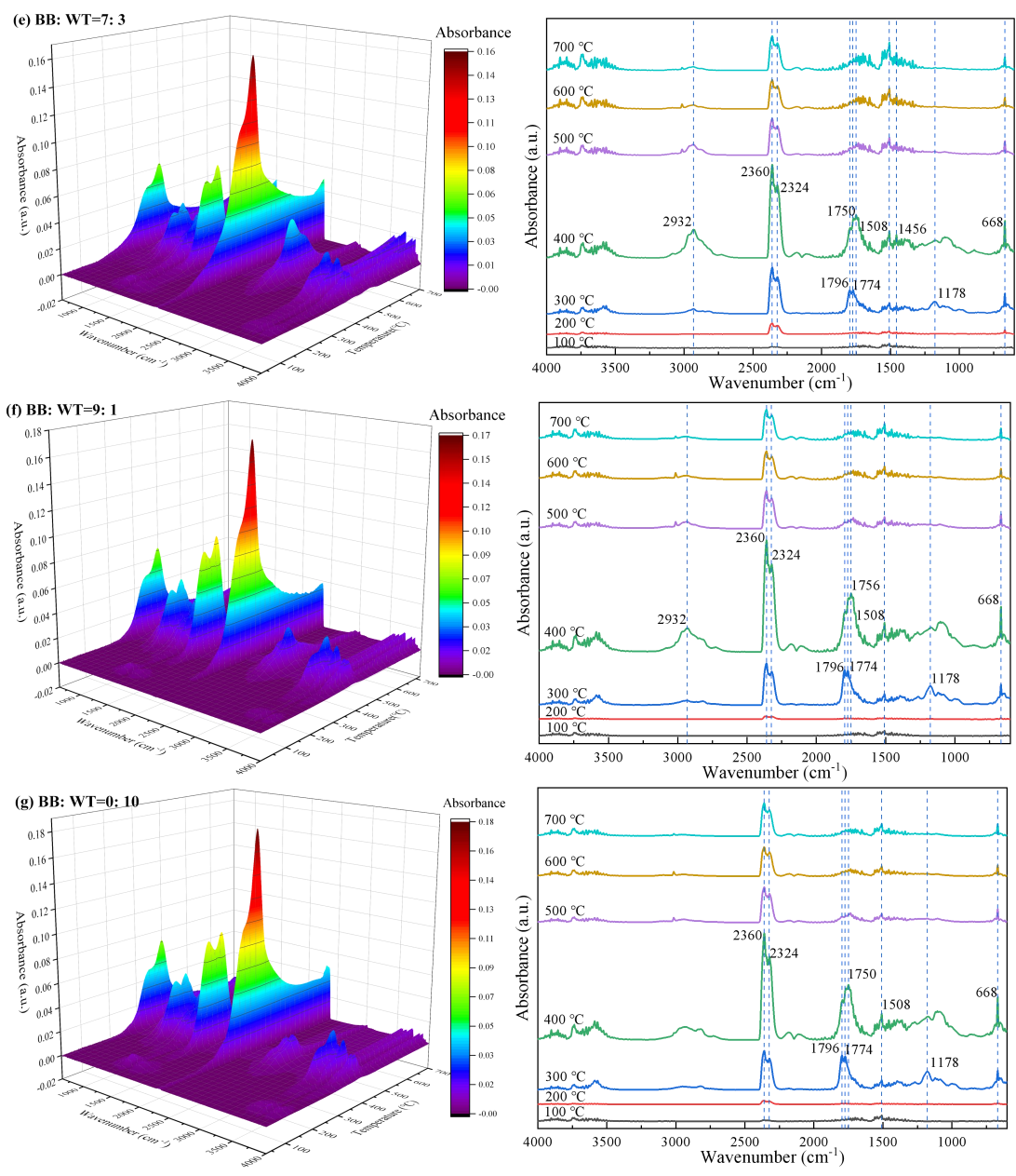
Fig.S2 The FTIR spectra during the co-pyrolysis of BB-WT blends.
