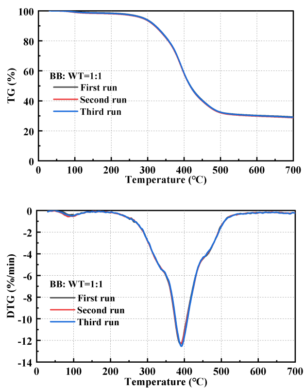
Fig.S1 TG and DTG curves of the 1:1 BB-WT blend obtained from three repeated runs.
