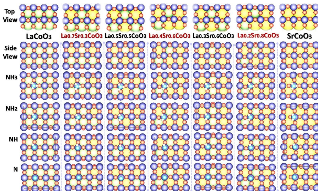
Fig. S1: The atomic structure for each model catalyst used in the DFT calculation
