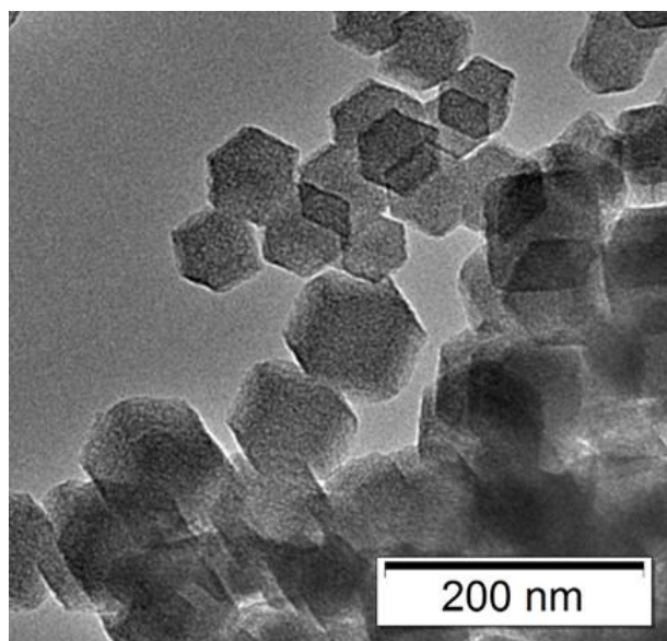
Fig. S1 TEM image of ZIF-67.
