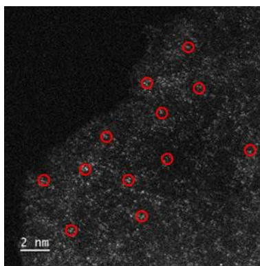
Fig. S3 HAADF-STEM image of Co SACs.
