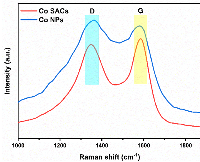
Fig. S4 The Raman shift of Co NPs and Co SACs.
