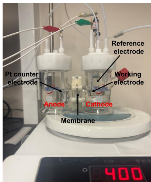
Fig. S5 Photograph of the H-cell setup used for nitrate reduction experiments, showing the working, counter, and reference electrodes, and the ion exchange membrane separating the electrolyte compartments.
