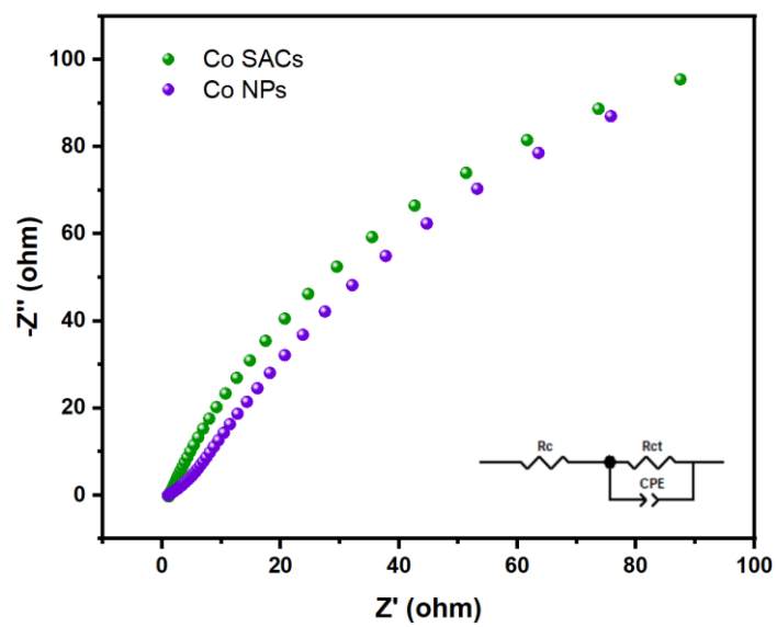
Fig. S6 Nyquist plots for EIS charge transfer resistance tests of Co SACs and Co NPs.
