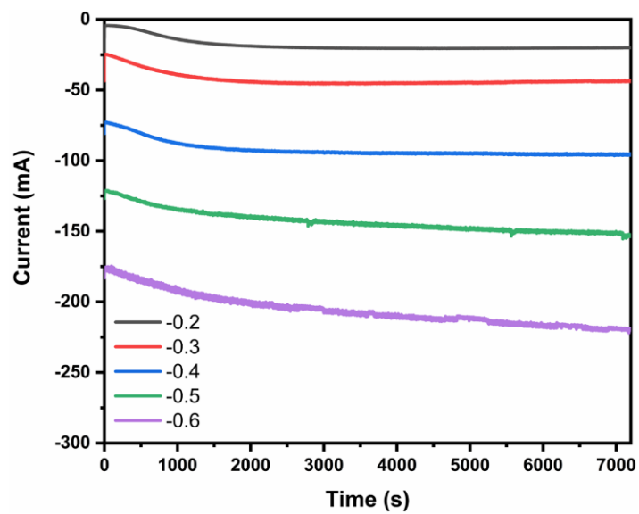
Fig. S7 The i-t curve of Co NPs electrocatalyzing NO 3 RR for 2 hours at -0.2 to -0.6V vs. RHE.
