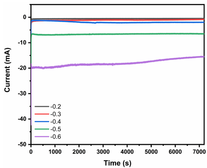
Fig. S9 The i-t curve of NC electrocatalyzing NO 3 RR for 2 hours at -0.2 to -0.6V vs. RHE.
