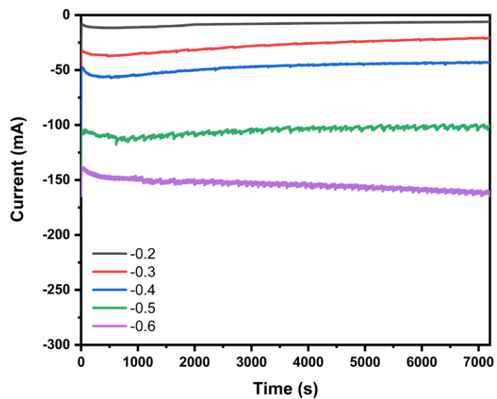
Fig. S8 The i-t curve of Co SACs electrocatalyzing NO 3 RR for 2 hours at -0.2 to -0.6V vs. RHE.
