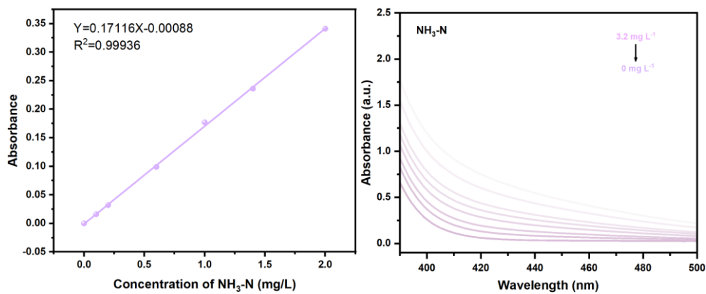
Fig. S10 Concentration-absorbance UV-visible calibration curves of NH 3 -N.
