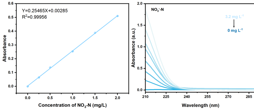
Fig. S11 Concentration-absorbance UV-visible calibration curves of NO 3 -N.
