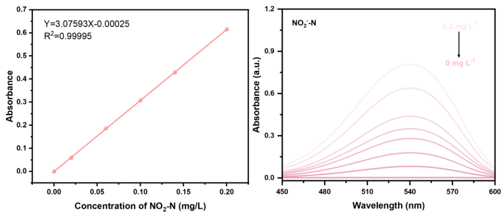
Fig. S12 Concentration-absorbance UV-visible calibration curves of NO 2 -N.
