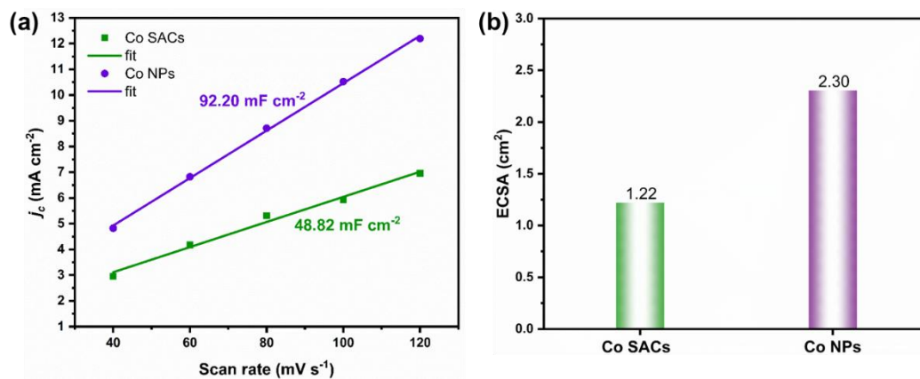
Fig. S14 (a) Plots of the current density versus the scan rate for Co SACs and Co NPs. (b) Electrochemical surface area (ECSA) of Co SACs and Co NPs. The double-layer capacitance ( C_{dl} ) is proportional to the ECSA.
