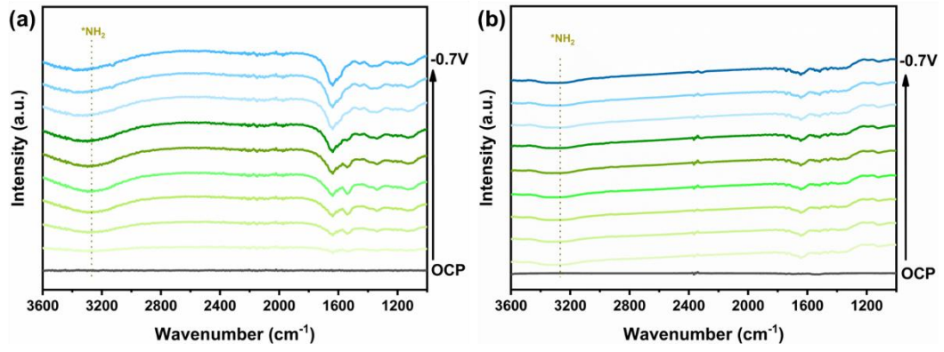
Fig. S15 Operando ATR-FTIR spectra of Co NPs (a) and Co SACs (b) at various applied potentials.
