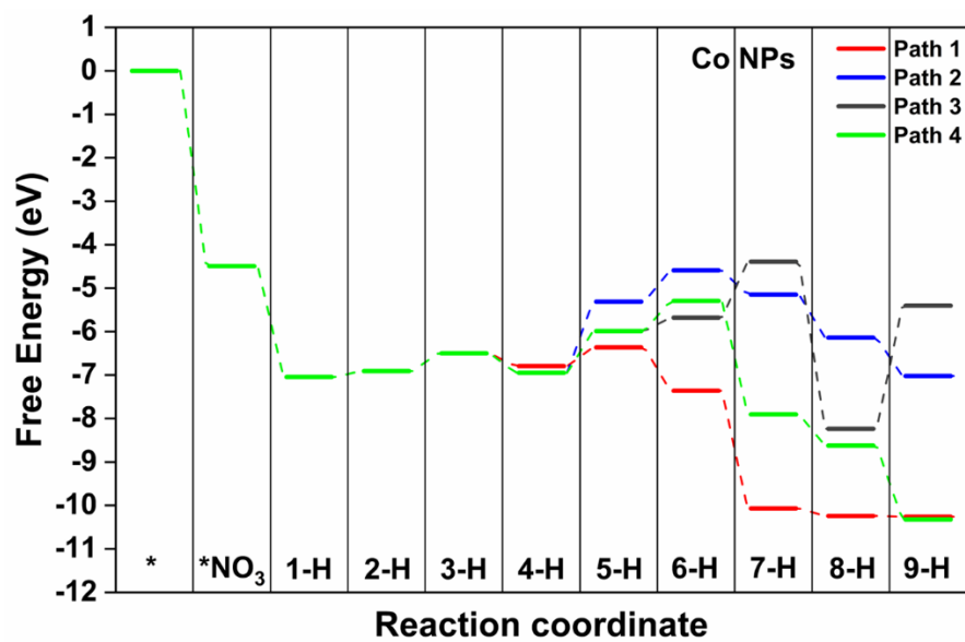
Fig. S16 Reaction barrier diagrams of the four reaction pathways of Co NPs.
