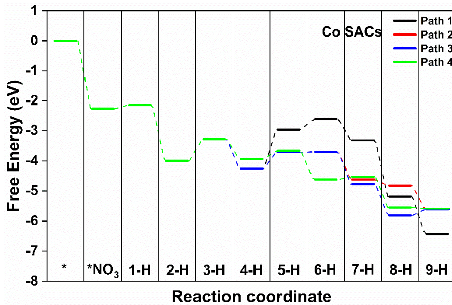
Fig. S17 Reaction barrier diagrams of the four reaction pathways of Co SACs.
