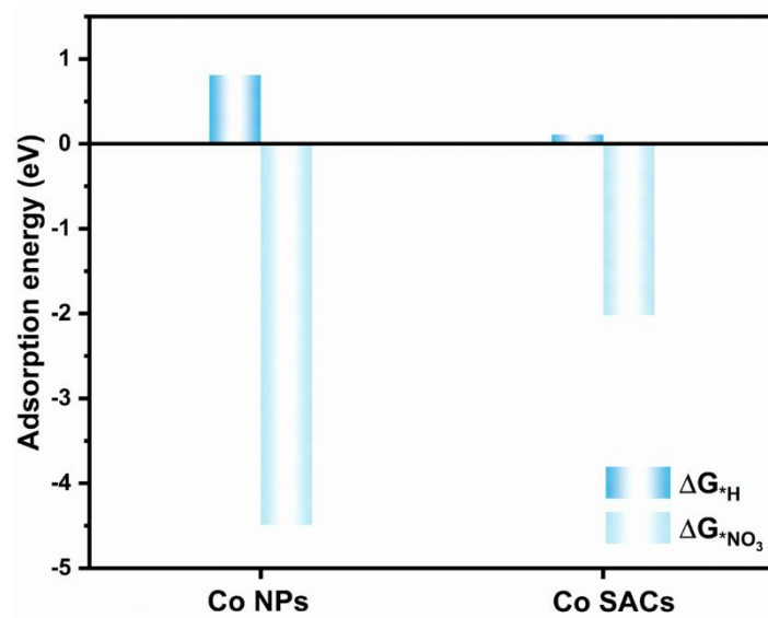
Fig. S18 The adsorption energy of Co NPs and Co SACs for *H and *NO 3 .
