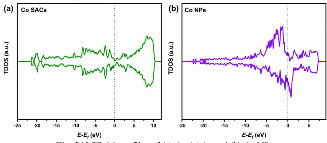
Fig. S19 TDOS profiles of (a) Co SACs and (b) Co NPs.
