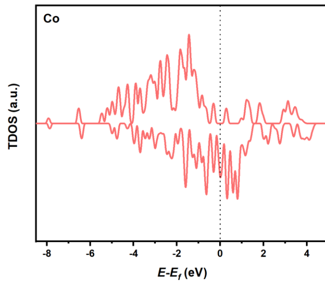
Fig. S20 TDOS profiles of Co NPs without nitrogen-doped carbon substrate.
